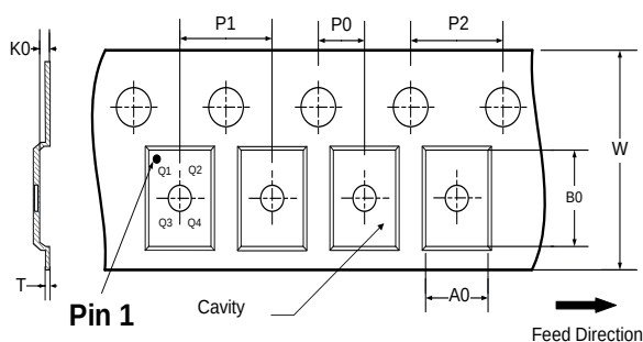
TAPE DIMENSIONS
